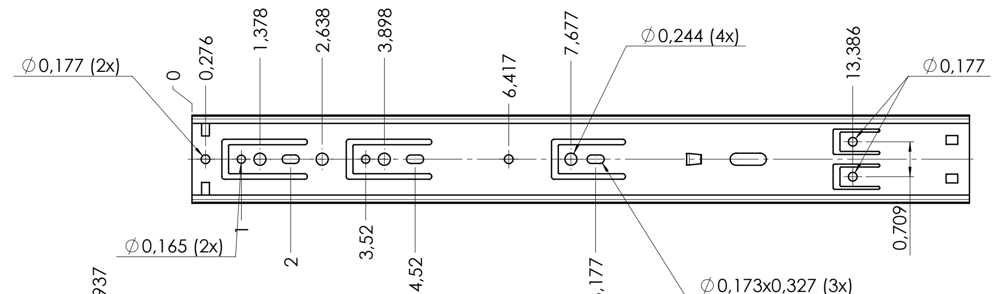
CABINET MOUNTING HOLES
