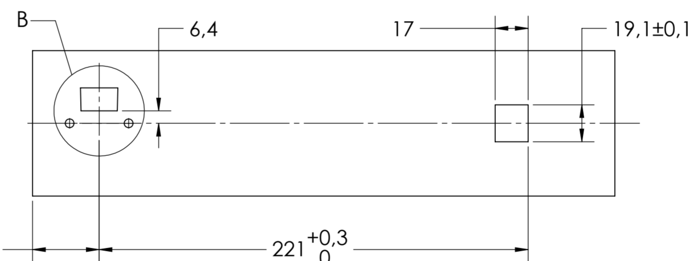
CABINET MOUNTING CUTOUTS
