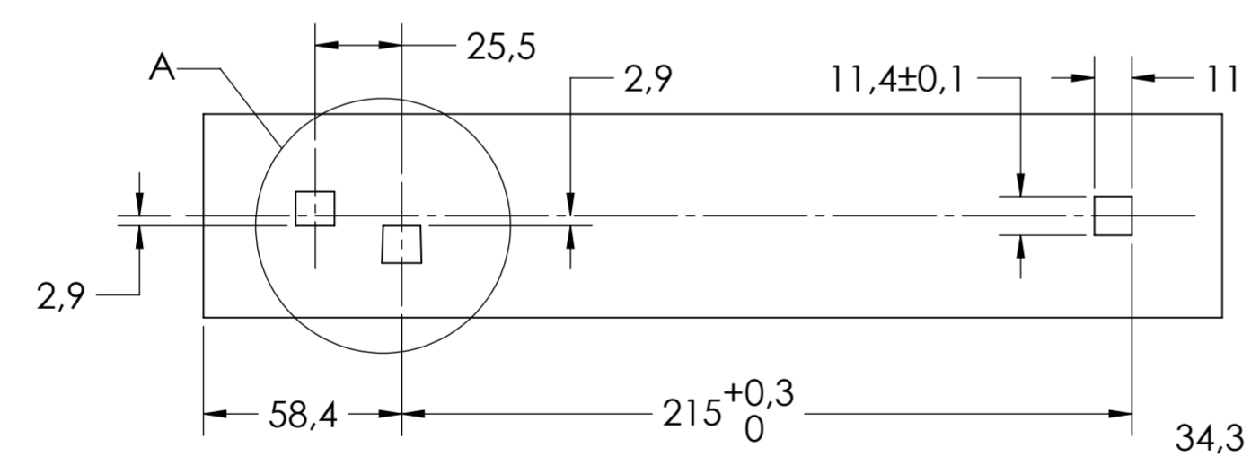
DRAWER MOUNTING CUTOUTS
