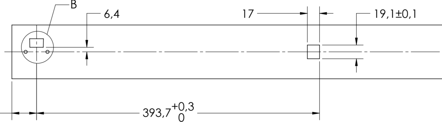
CABINET MOUNTING CUTOUTS
