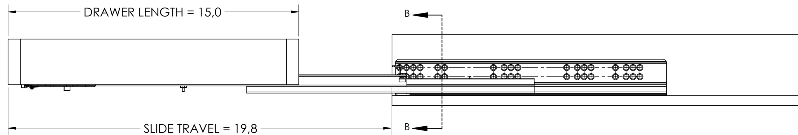
LOCKING KIT BOTTOM MOUNT SCALE 1:1.5
