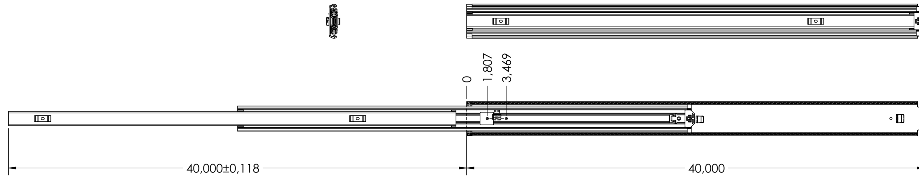
DRAWER MOUNTING CUTOUTS
